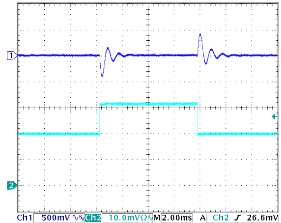
Figure 16: Output voltage response to step-change in load current (50%-75%-50% of I_{out(max)} ; dI/dt = 5A/\mu s ). Load cap: 470 \mu F , 30 mW ESR tantalum cap and 1 \mu F ceramic cap. Ch 1: Vout (500mV/div), Ch 2: Iout (2A/div).
