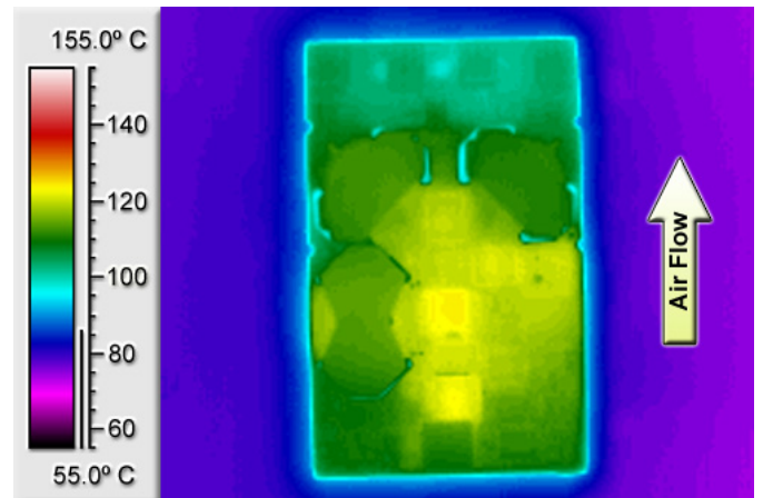
Figure 12: Thermal plot of converter at 6.0 amp load current with 85°C air flowing at the rate of 200 LFM. Air is flowing across the converter from input to output (48V input).
