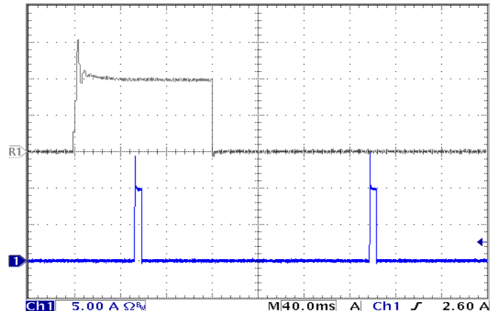
Figure 22: Load current (5 A/div) as a function of time when the converter attempts to turn on into a 10 mW short circuit. Top trace (40 ms/div) is an expansion of the on-time portion of the bottom trace.
