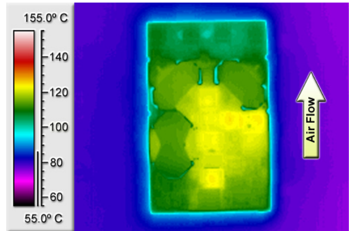
Figure 10: Thermal plot of converter at 6.5 amp load current with 85°C air flowing at the rate of 200 LFM. Air is flowing across the converter from input to output (24V input).
